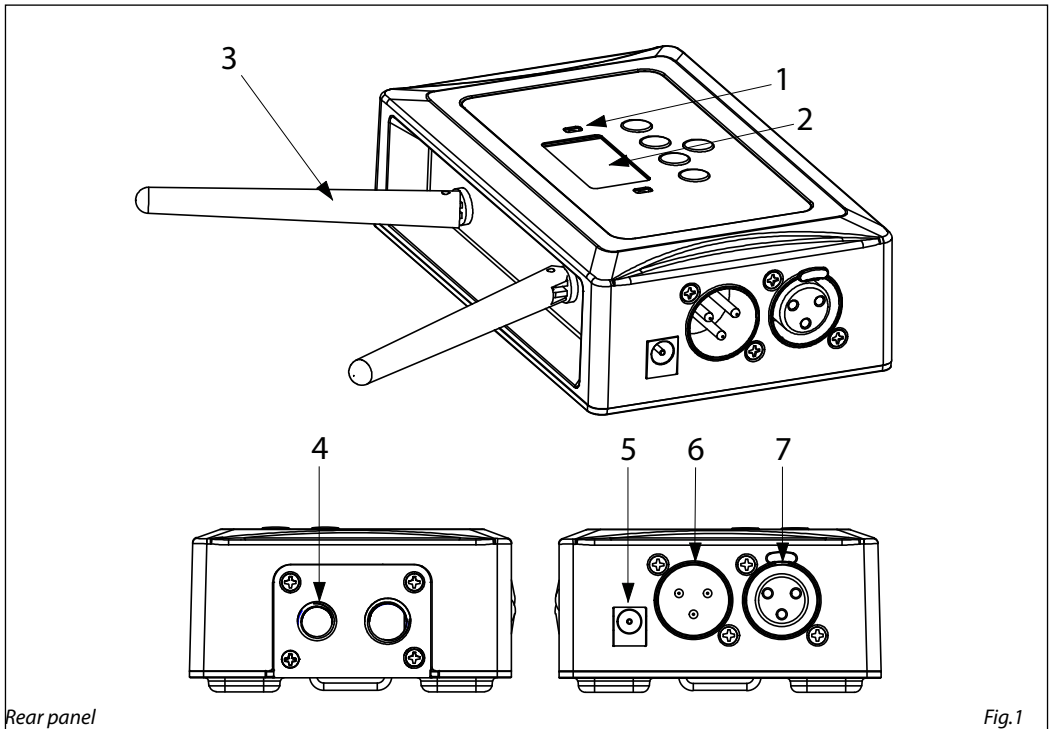
Rear panel
